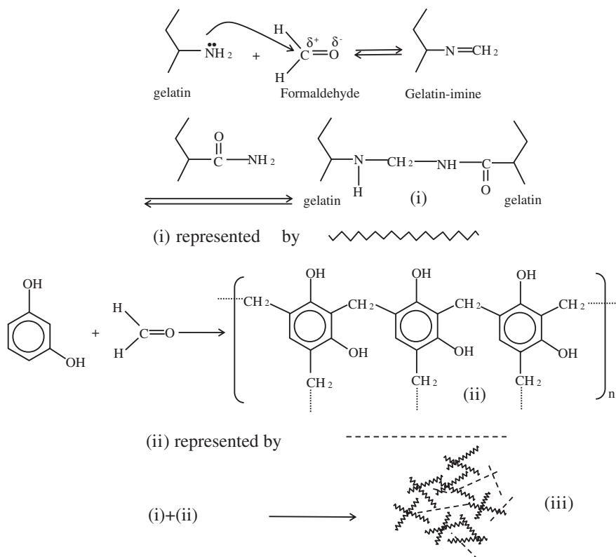
Fig. 8.2 Reaction scheme for gelatin-resorcinol-formaldehyde (GRF) glue
