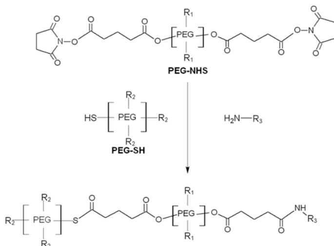
Fig. 8.4 Reaction scheme for CoSeal®
