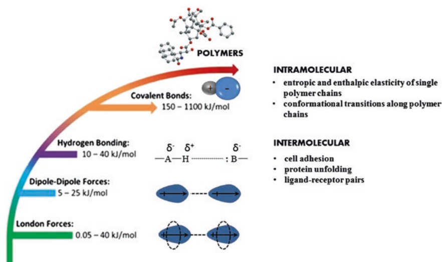
Fig. 3.1 Intramolecular and Intermolecular forces in polymers for biomedical use
