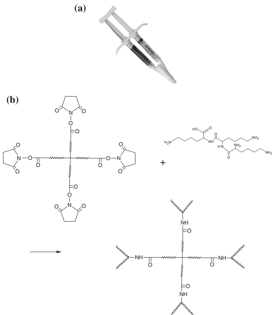
Fig. 8.3 a DuraSeal TM applicator and b reaction scheme for DuraSeal TM
